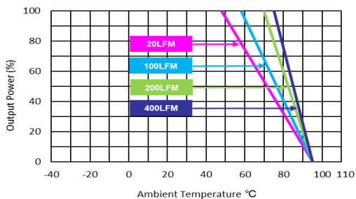
MKE20-12S05HI, MKE20-12S051HI
