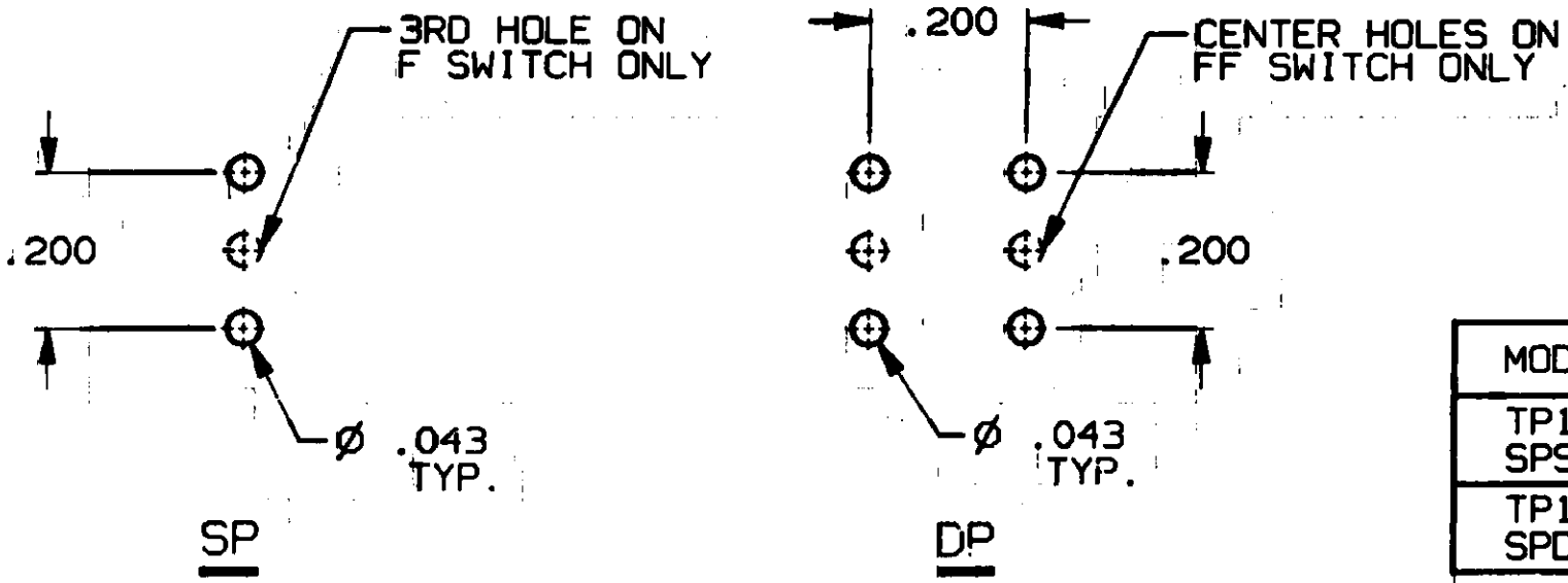
RECOMMENDED HOLE LAYOUT TOLERANCE ± .002 UNLESS OTHERWISE NOTED
