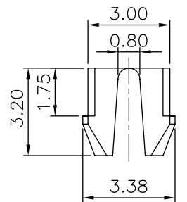
DETAIL X
