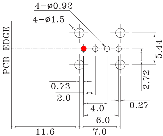
PC Board Layout - Bottom View
