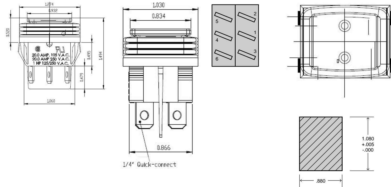
Panel Cut Out Panel Thickness 1/32" - 3/16"
