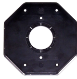
WP107 Double-Gang Round Insert, 1 3/8", 1 5/8", 1 3/4"
