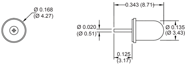
Part Number: CW1600-3
