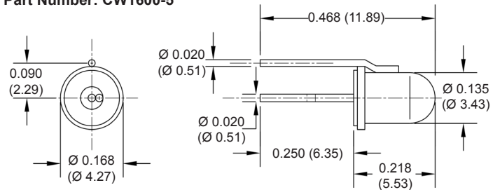
Part Number: CW1600-5
