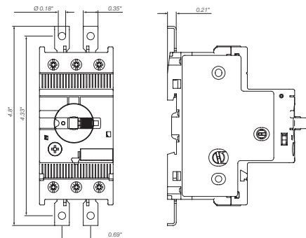
MS132-T > 10 A with screw fixing kit FS116 (accessory)
