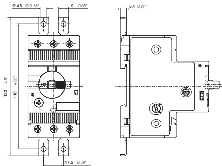
MS132-T ≤ 10 A with screw fixing kit FS116 (accessory)
